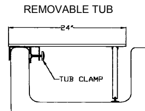
REMOVABLE TUB
